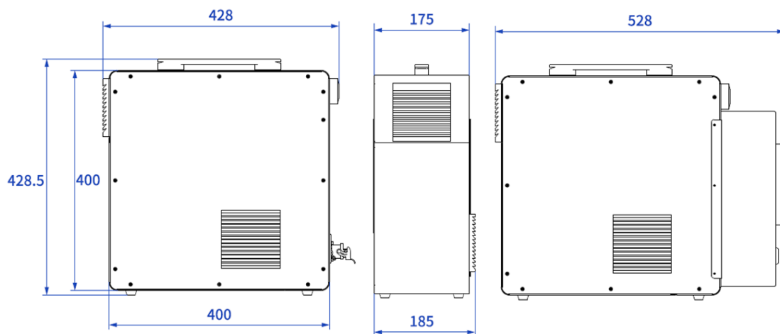
Figure 5.30 CC263 dimensions
