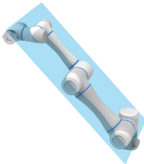
Figure 4.6 Elbow singularity
