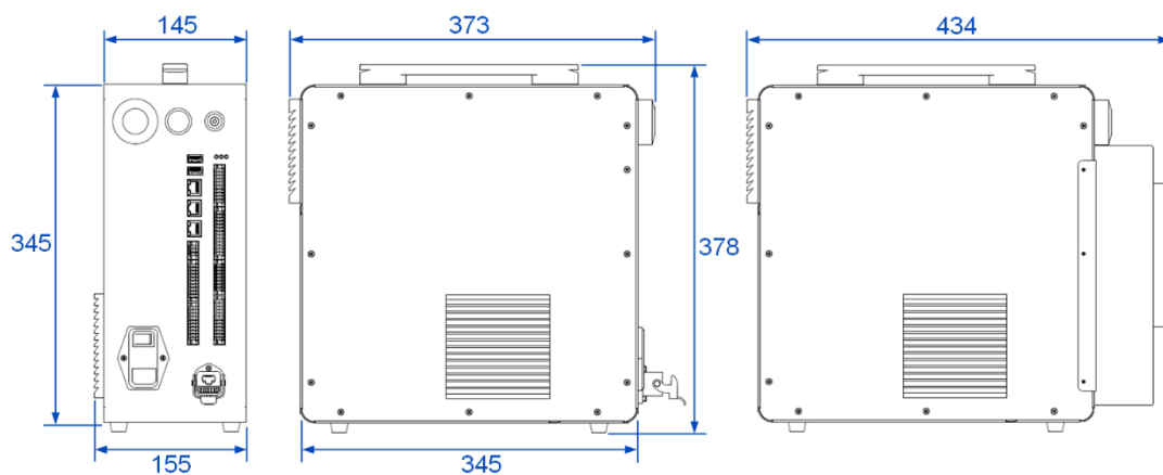
Figure 5.29 CC262 dimensions
