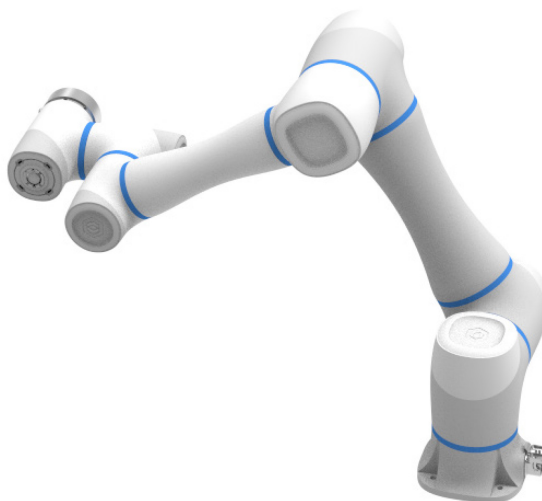
Figure 4.7 Wrist singularity
